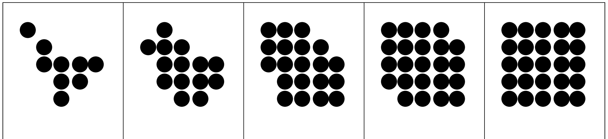
Filling the convex hull 9
