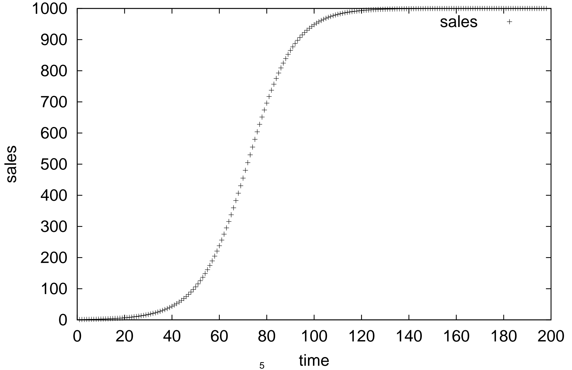
time plot of purchases r=2 M=1000
